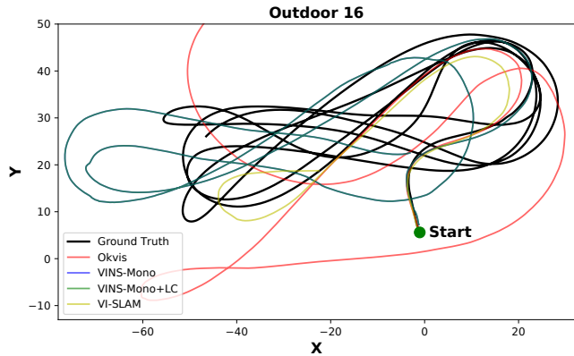
Fig. 8: Visual-inertial odometry results on the Outdoor 16 sequence. This is one of the faster outdoor sequences, flying several large figure eight laps around the open field. In this case, all of the algorithms (including Okvis [32] and VINS-Mono [31]) begin to drift on the second turn, and rapidly drift away from the ground truth trajectory. Qualcomm’s VI-SLAM is able to track closer to the true trajectory for a bit longer, but fails before completing a full lap.
